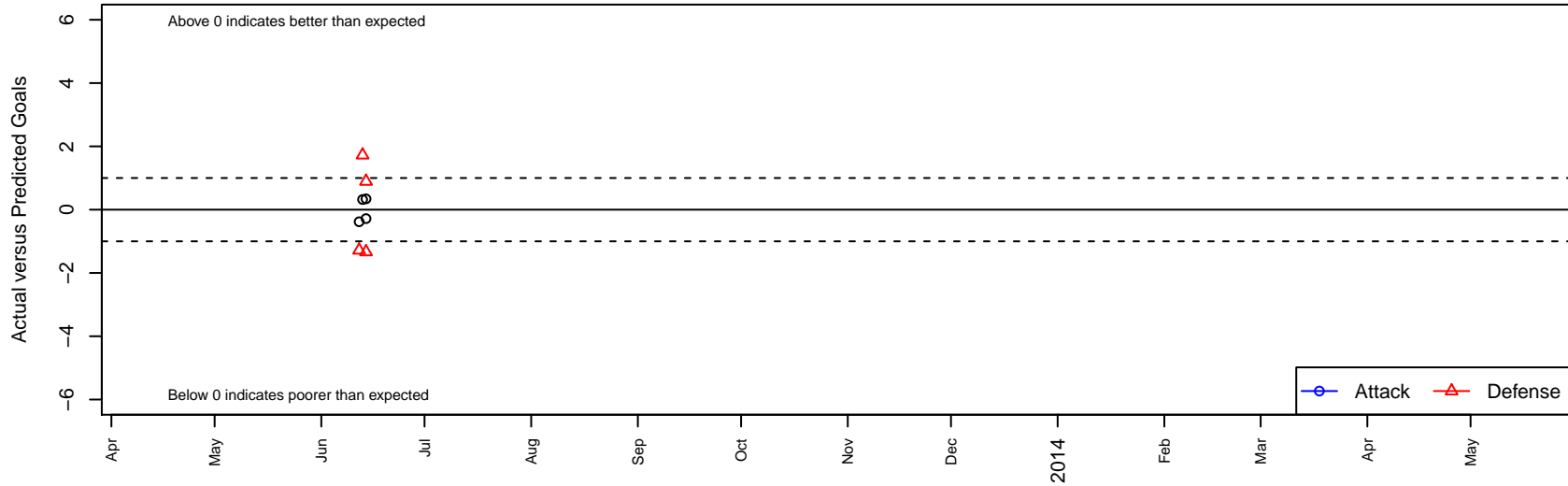
MSC United B97 Dots are actual minus expected GF (blue circles) and GA (red triangles). Blue line is smoothed change in attack strength. Red is smoothed change in defense strength.
